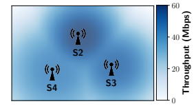
Fig. 10. DL tput. density in 60m×40m test area.
